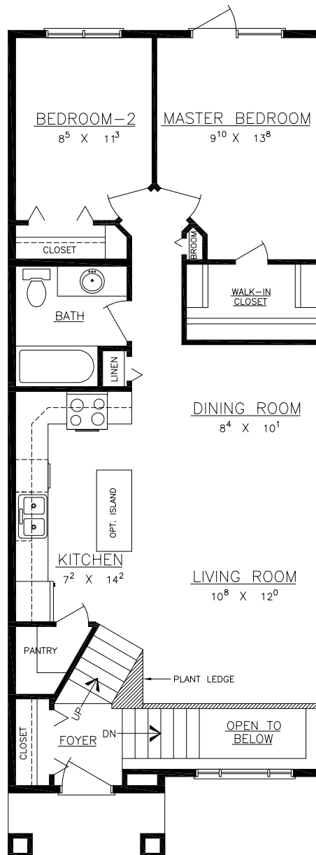
FLOOR PLAN
